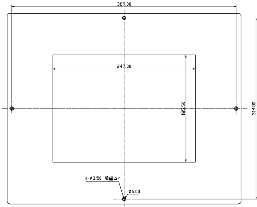
Panel-PC FlexLine 12": Frontpanel "Big"
