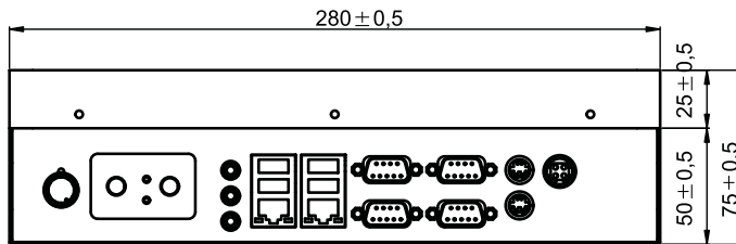
BOTTOM VIEW
